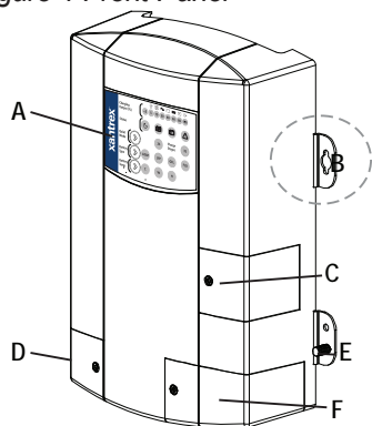
Figure 4 Front Panel
