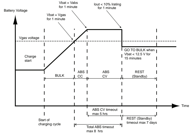
Figure 18 Two-Stage Charging Process
