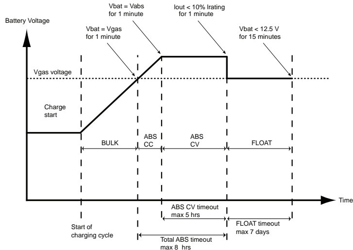
Figure 17 Three-Stage Charging Process
