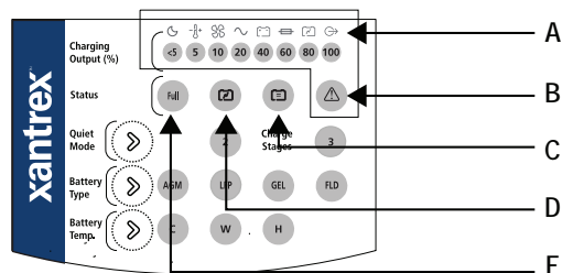
Figure 23 Charger and Battery Information
