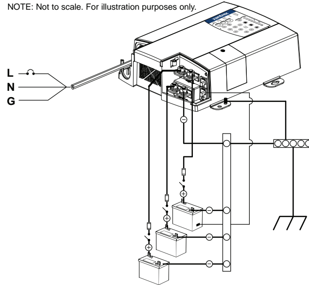
Figure 16 Typical Three-Battery Installation
